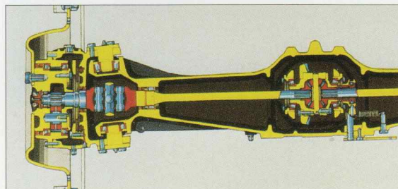
ALL-WHEEL DRIVE
