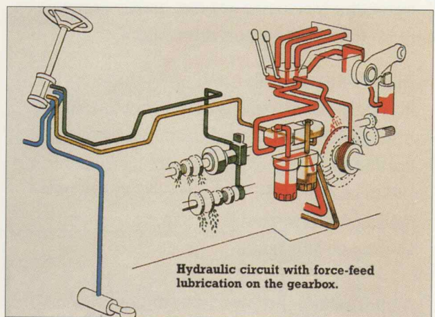
HYDRAULIC FLOW
