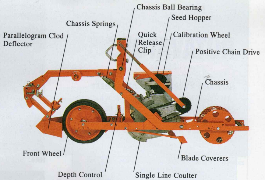
▲ SINGULAIRE 785 ROW UNIT Clod deflector and cage rear wheel are optional. Single or multi-line coulters available.
