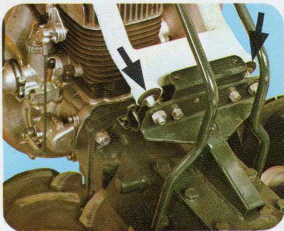
central bar, rubber-mounted
