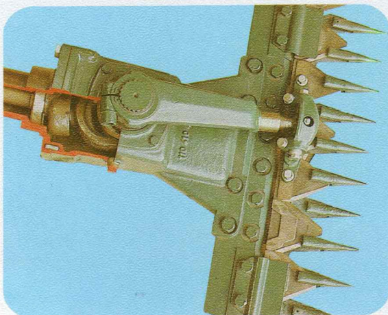
wear-resistant oilbath-mower drive with new, easy-to-maintain knife head
