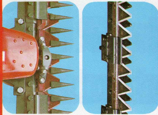
Medium cut (ill. left) bar and mulch bar (ill. right) are available, as well as fine cut- and non-stop bar
