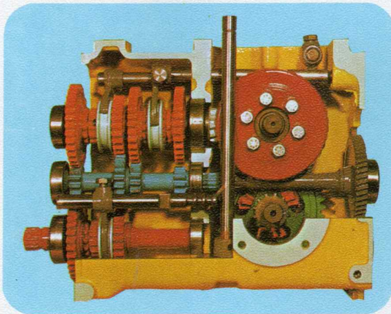
Type 112 with differential with lock
