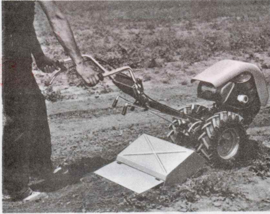
Rotary Hoe 52 cm working width with 16 blades — for a garden quality seed-bed.
