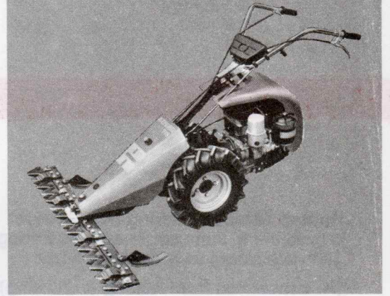
Motor mower with finger- or mulching cutter-bar, 1,10 m working width.
