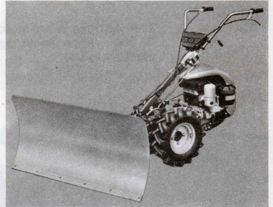
Snow-plough adjustable plough angle, 1 m working width.
