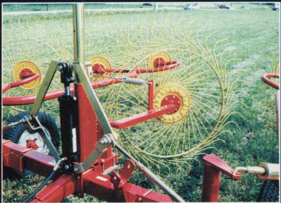
Hydraulic lift linkage assembly
