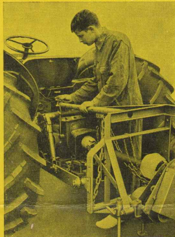
Mounting of the overload release for cutterbar on the drawbar bracket. Locking is simple, fast and safe.
