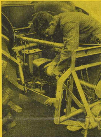
The upper link tube is attached to the tractor.
