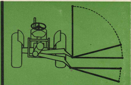
The AKTIV TH has a large working area. The cutter bar can be varied \pm 15^\circ in relation to ground level, so that sloping sides of ditches, highway embankments and similar banks can be efficiently cut. The cutter bar is positioned by means of the tractor's hydraulics. No hydraulic brackets required on the mower.
