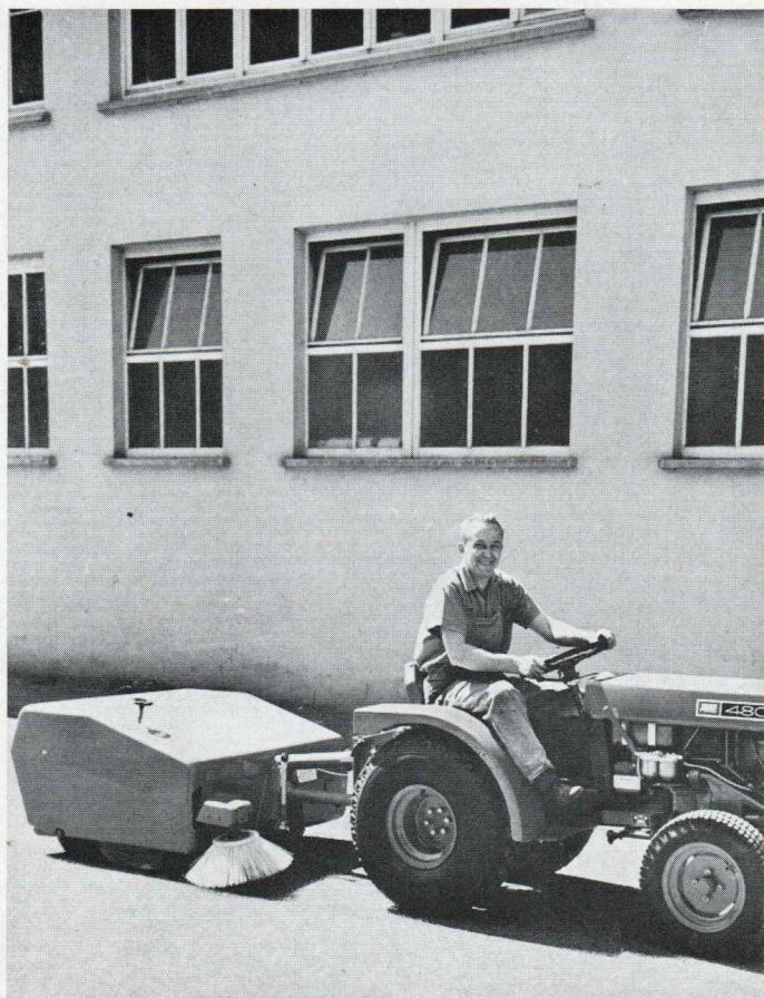
For sweeping and simultaneous collection of rubbish, this trailed sweeper with 100 ltr. (22 gals.) capacity rubbish container is available. The sweeper roll is 100 cms. (39 ins.) long and 40 cms. (16 ins.) in dia. With the gutter brush in addition, the total working width is approx. 125 cms. (49 ins.).
