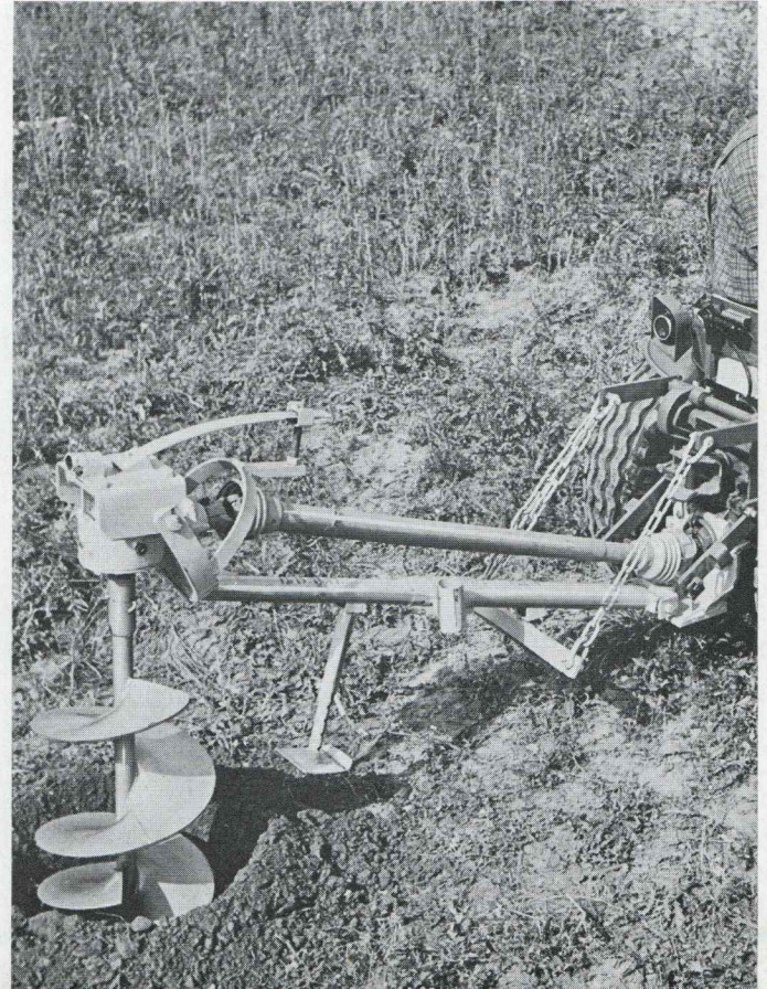
The earth auger too, is a much used attachment. Various augers are available with 110, 160, 250 and 400 mms. dia. (4.3, 6.3, 9.8, 15.7 ins.). Performance: approx. 150-220 borings per hour, depending on auger dia. and nature of ground.
